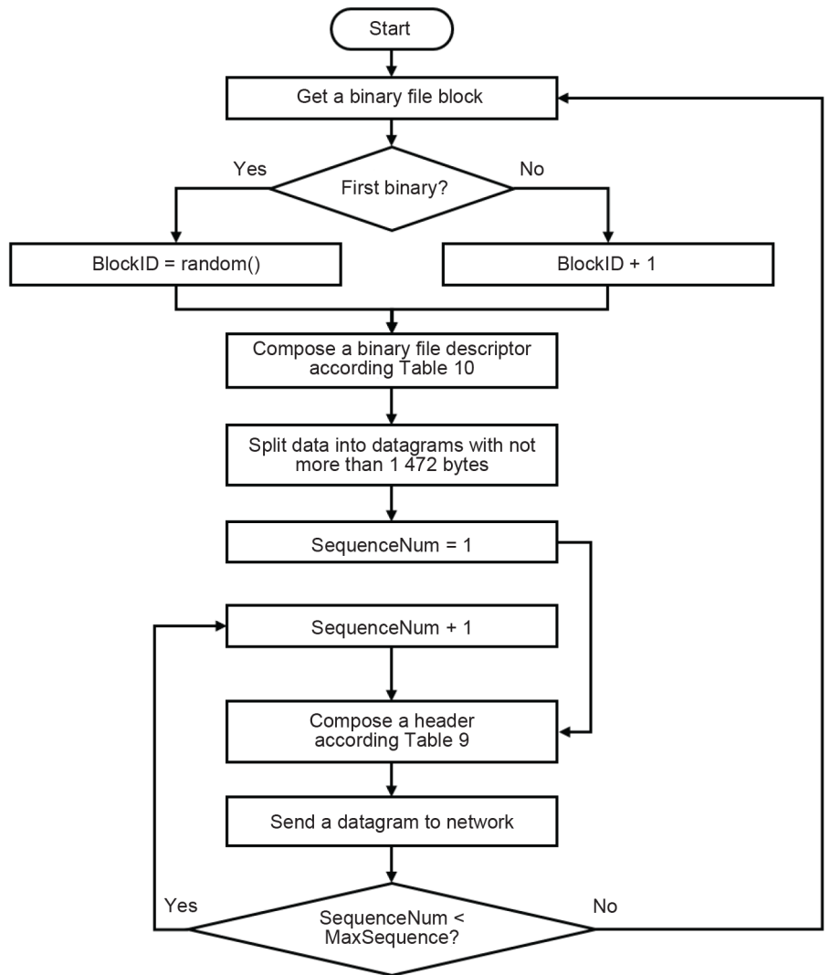
Figure 5 – Non re-transmittable sender process
